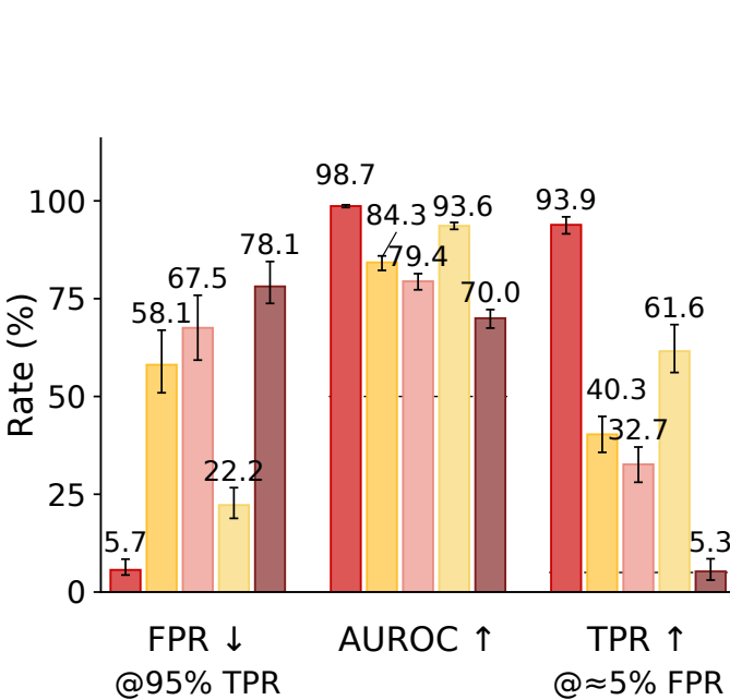
(a) Null-aware
