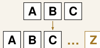
(c) Option-scalable
