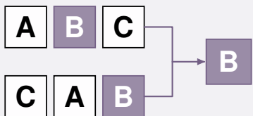
(b) Permutation-invariant
